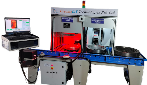
VISION BASED CONVEYOR SYSTEM FOR FLYWHEEL
