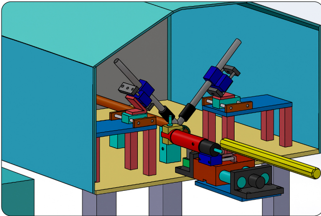
SERVO CONTROLLED CO2 WELDING MACHINE AUTOMATION
