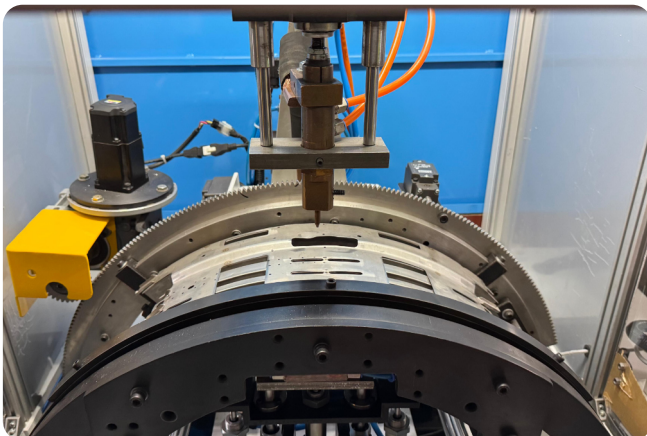
SPOT WELDING SPM AUTOMATION FOR AEROSPACE COMPONENTS
