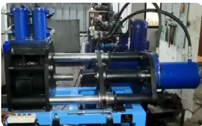
TUBE END SWAGING MACHINE
